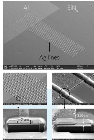
Fig. 2. SEM images of printed conductive line
